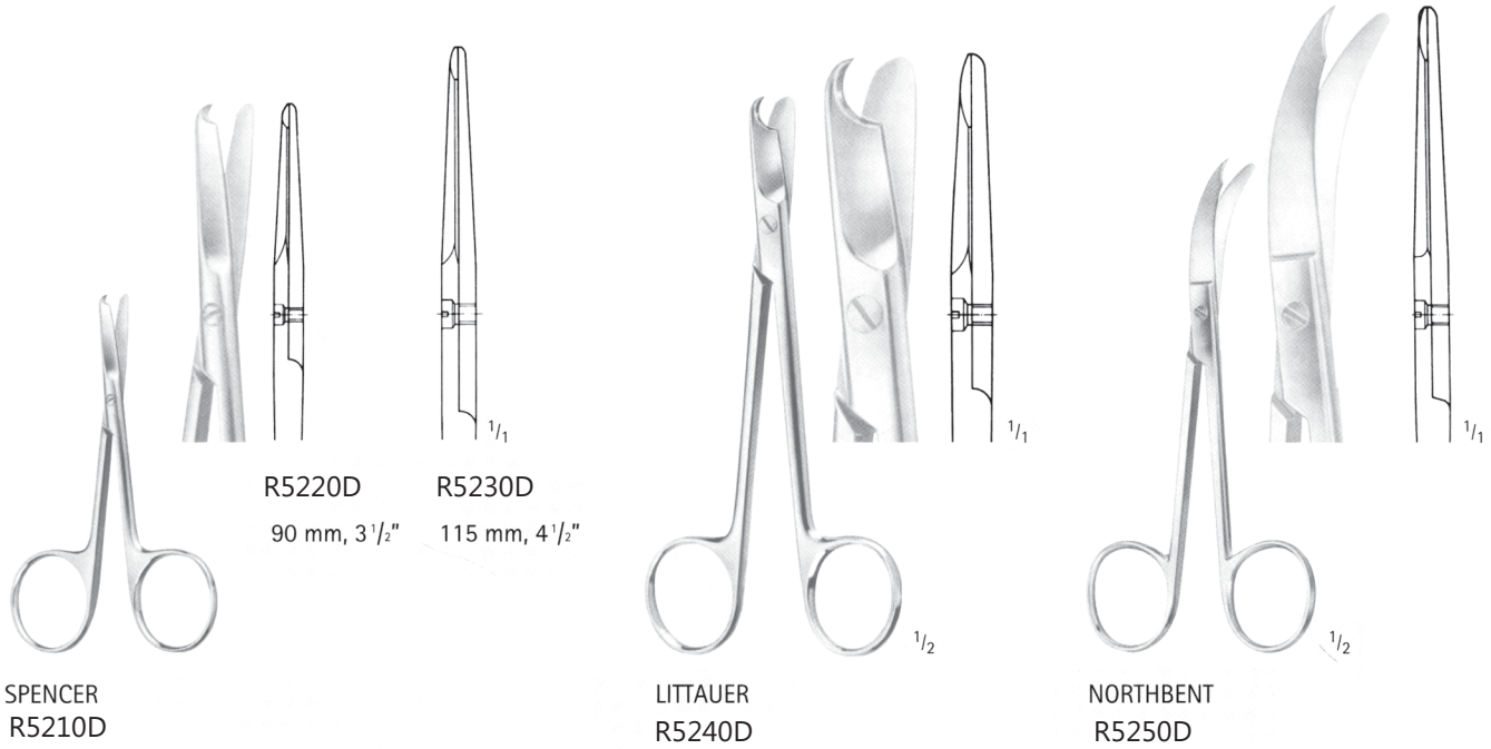
Ligature scissors
